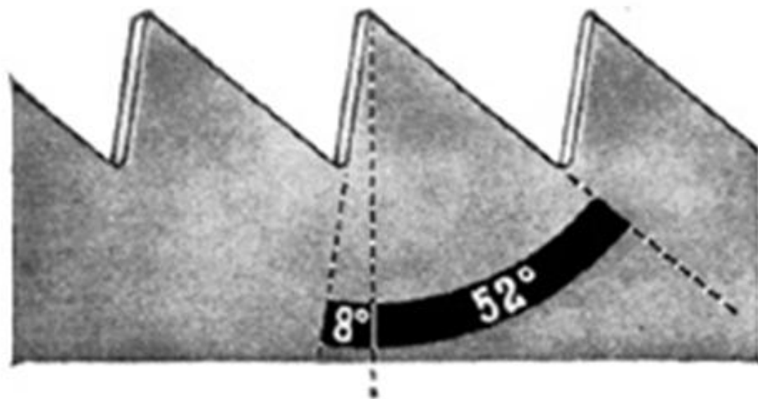
Side view of rip teeth (enlarged)
