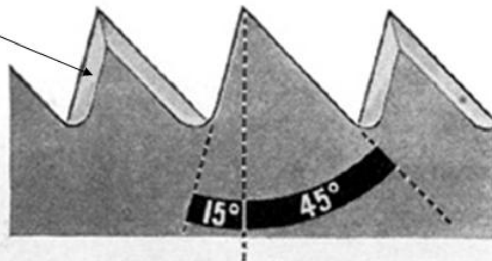
Side view of cross-cut teeth (enlarged)
